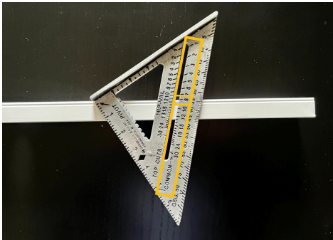
Example of Measuring cut for an 8/12 Roof Pitch
